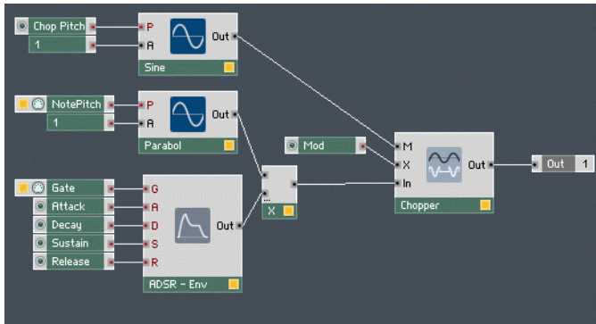
Fig. 12.16 The Structure for a chopper distortion effect.
