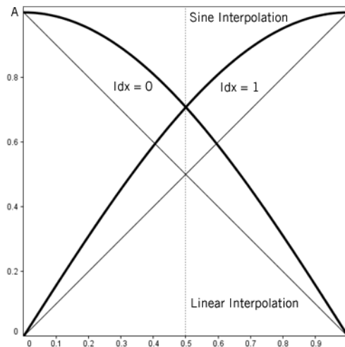
Fig. 5.16 Crossfading curves for linear and sine interpolation.
