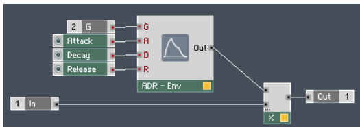
Fig. 9.35 A simple implementation of an attack-decay-release envelope.
