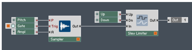
Fig. 12.33 The Slew Limiter traces the signal incoming from the Sampler Module, depending on the slew rates set at the "Up" and "Down" input ports.
