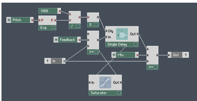
Fig. 11.3 The Structure of a comb filter.
