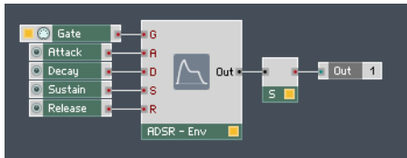
Fig. 14.39 Use the Event smoother Module to convert the Audio signal from the ADSR Module to a smoothed Event signal running at the Control Rate.
