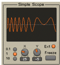
Fig. 6.46 An example of a frequency modulated sine waveform.
