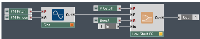
Fig. 10.37 A simple implementation of a low shelving filter.
