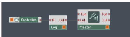
Fig. 2.37 The Controller Module can be used to send specific MIDI Controller messages to parts of your Structure, such as the "Lvl" input port of the Master Tune/Level Module.
