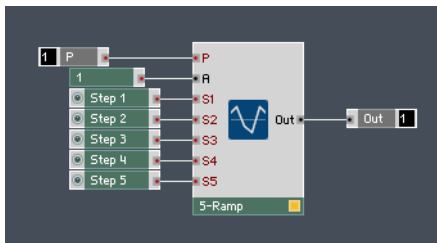
Fig. 6.99 A simple implementation of the 5-Ramp Module.
