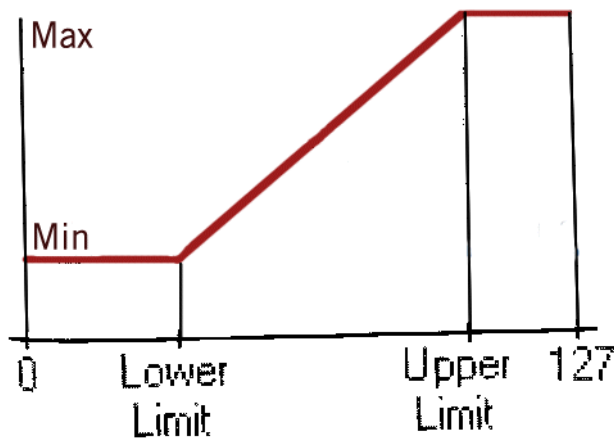
Fig. 2.31 The x-axis of the graph shows the incoming MIDI values whereas the y-axis shows the outgoing release velocity values from the Off Velocity Module. The values are interpolated linearly between “Min” and “Max”.
