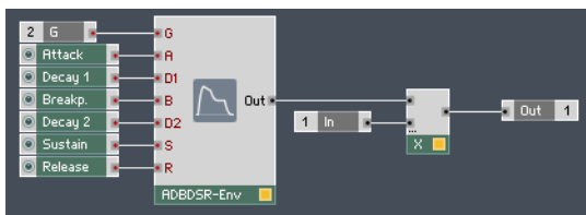
Fig. 9.44 A simple implementation of an attack-decay-breakpoint-decay-sustain-release envelope.
