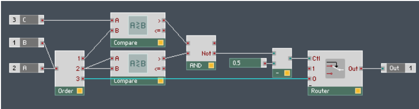
Fig. 13.47 Compare and Logic Modules can be used to determine whether a signal is to be forwarded by a Router Module or not.
