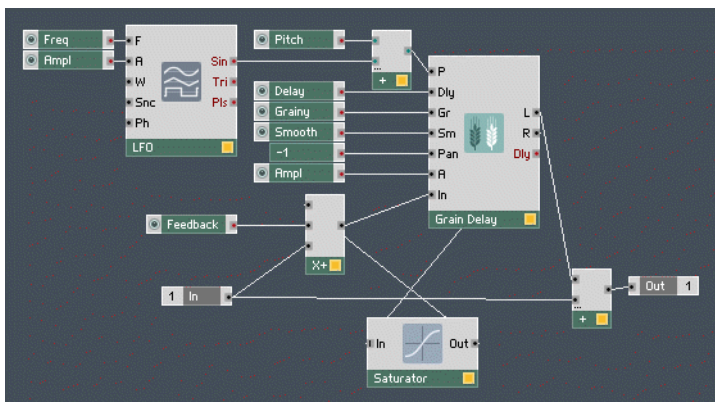
Fig. 11.11 The Structure of a simple pitch shifter delay effect.
