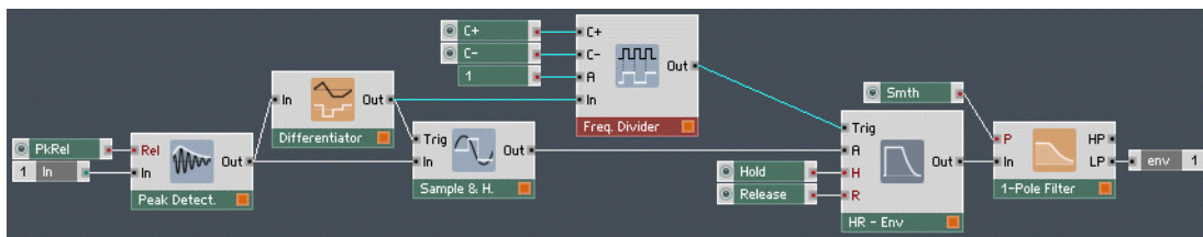
Fig. 12.40 In this modified envelope follower Structure, the Frequency Divider Module lets you filter out positive zero crossings which trigger the HR Envelope Module.
