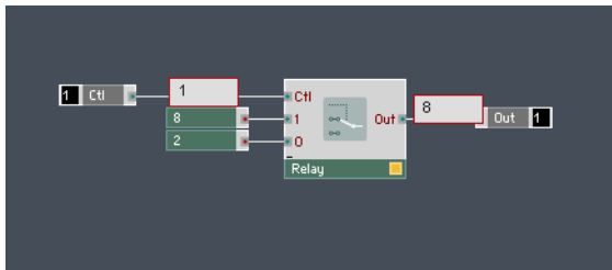
Fig. 5.8 A "Ctl" value of "1" at the corresponding Relay input port causes the value at the upper "channel" input port to be forwarded to the Relay Module's output.
