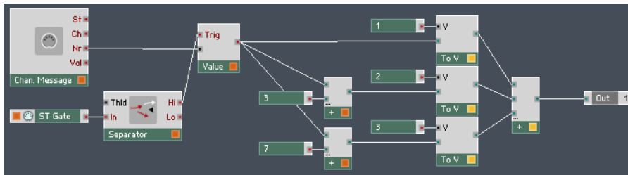
Fig. 2.17 The Structure to create a chord from an incoming Monophonic MIDI Note.
