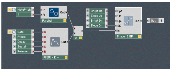
Fig. 12.22 The Structure for a waveshaping effect with two breakpoints.
