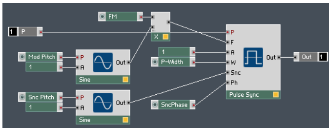
Fig. 6.63 A simple implementation of the Pulse Sync Module.
