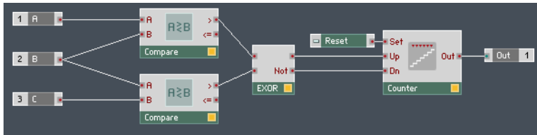
Fig. 13.26 Compare, Logic, and Counter Modules make a useful combination for algorithmic sequencing.
