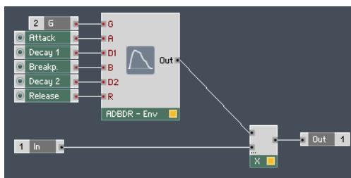
Fig. 9.41 A simple implementation of an attack-decay-breakpoint-decay-release envelope.
