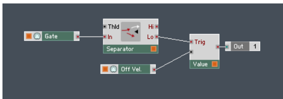
Fig. 2.33 The Structure for sending a Gate Off Event with Velocity Off value.
