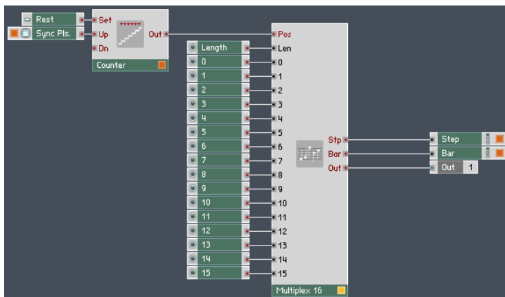
Fig. 2.56 16 step sequencer
