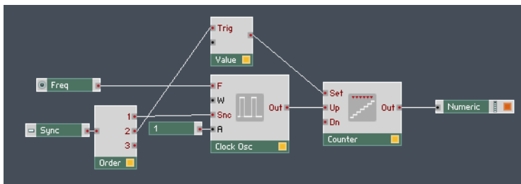
Fig. 6.110 This Structure is an implementation of a simple timer.
