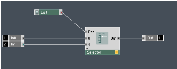
Fig. 1.7 Here you see a common Structure for routing signals. Here, a List Module is used to supply the “position” value the “Pos” input port of a Selector Module.
