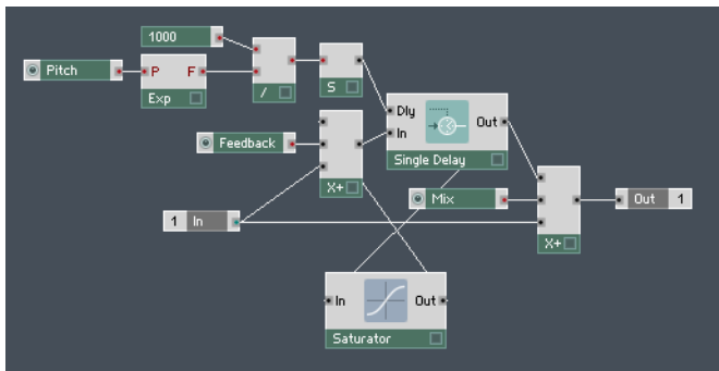
Fig. 14.37 The Structure of a comb filter.
