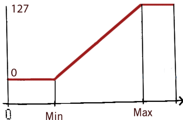
Fig. 3.8 The x-axis of the graph shows the values at the input port whereas the y-axis shows the outgoing MIDI CC message values. These values are interpolated linearly between over the interval [Min ... Max].
