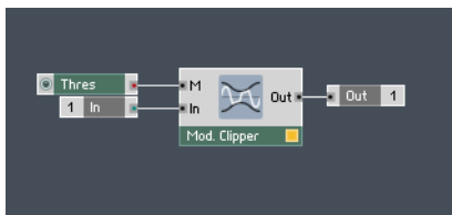
Fig. 12.8 The Structure for the hard clipper effect.
