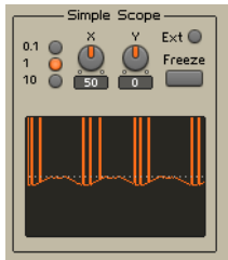
Fig. 6.82 An example of a hard synchronized impulse waveform.
