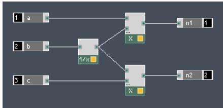
Fig. 4.18 One possible use for the Reciprocal Module is to normalize two signals with the same scaling factor.
