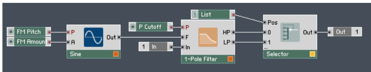
Fig. 10.4 A simple implementation of a 1-pole filter.
