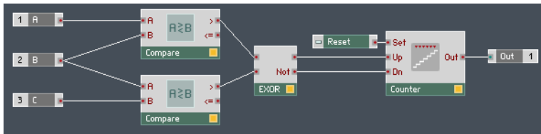
Fig. 13.4 Compare, Logic, and Counter Modules make a useful combination for algorithmic sequencing.
