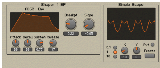
Fig. 12.20 The resulting waveform of a parabolic oscillator sent through a waveshaper with one breakpoint. Note the similarity to the Mirror 1 Module's effect on the same input signal.
