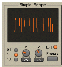
Fig. 6.67 An example of the output waveform of a frequency modulated Pulse 1-Ramp Module.
