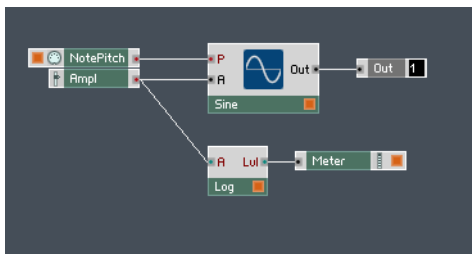
Fig. 4.37 The Log (A-to-Lvl) Module is used to convert linear amplitude values to logarithmic level values as displayed by the Meter Module.
