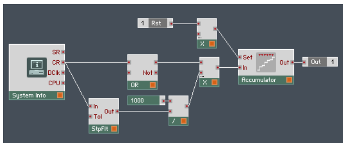
Fig. 14.57 The Structure for a simple Control Rate stopwatch.
