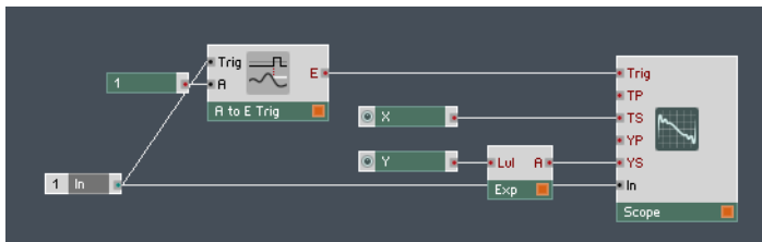
Fig. 14.22 The Structure for a simple scope that displays a Monophonic periodic Audio signal with regular zero crossings.
