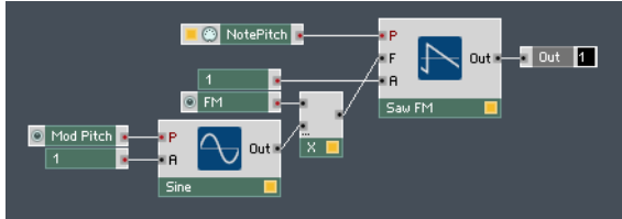
Fig. 6.5 A simple implementation of the Saw FM Module.
