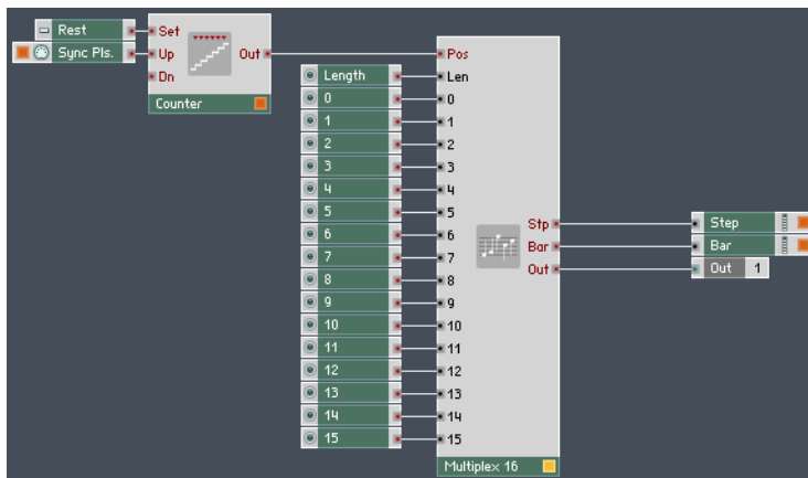
Fig. 1.46 Multiplex Sequencer
