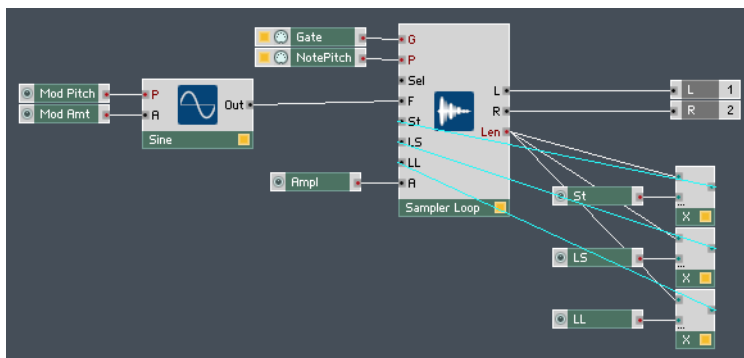
Fig. 2.12 The Structure for a frequency modulated loop sampler Instrument.
