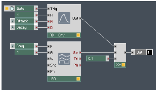
Fig. 4.15 You can use the Mult/Add Module on a signal to modulate it with an offset.
