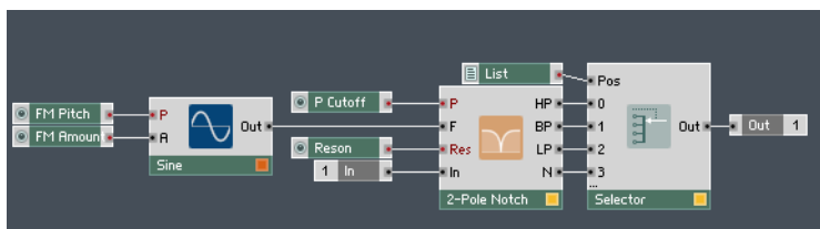
Fig. 10.12 A simple implementation of a 2-pole notch filter.
