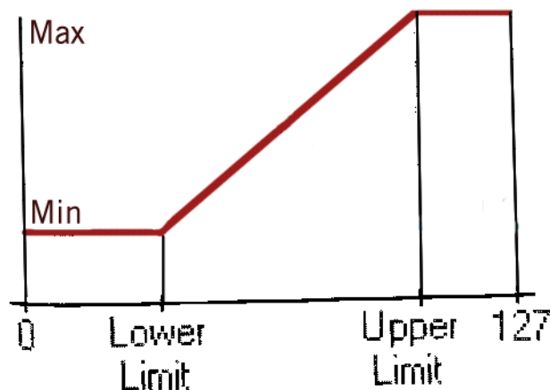
Fig. 2.20 The x-axis of the graph shows the incoming MIDI values whereas the y-axis shows the outgoing values from the Sel Note Gate Module. The values are interpolated linearly between “Min” and “Max.”
