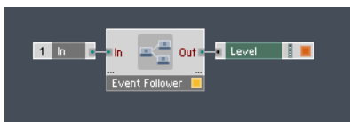
Fig. 1.26 The Level Meter Module displays the signal level from the "Event Follower" Macro, which is in the range [0 ... 1], in the logarithmic scale.
