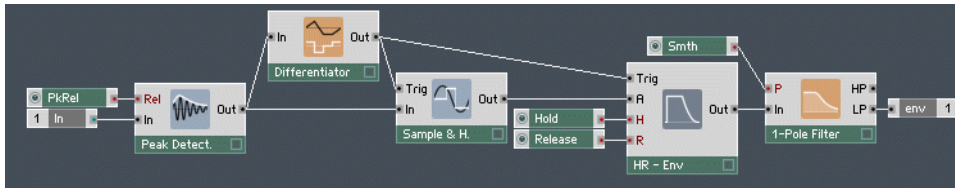
Fig. 12.38 The Structure for an envelope follower effect.
