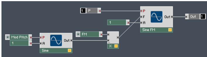
Fig. 6.45 A simple implementation of the Sine FM Module.
