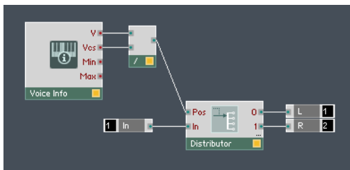
Fig. 14.50 The Voices in the Polyphonic signal sent from the "V" output port of the Voice Info Module carry their Voice number as their values. Dividing those values by the number of Voices yields a Polyphonic signal where each Voice carries a value in the range [0...1].
