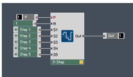
Fig. 6.87 A simple implementation of the 5-Step Module.
