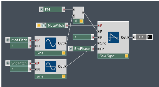
Fig. 6.8 A simple implementation of the Saw Sync Module.
