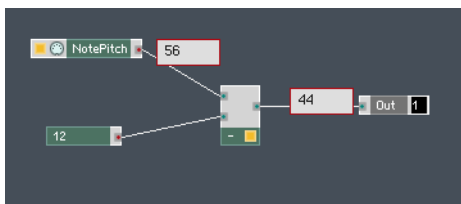
Fig. 4.7 In this example the Subtract Module is used to transpose the incoming pitch down 12 semitones.
