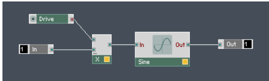
Fig. 4.48 A common application for the trigonometric sine function is found in waveshaping.
