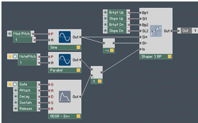
Fig. 12.25 The Structure for a waveshaping effect with three breakpoints and Audio Rate modulation for two of the four slope parameters.
