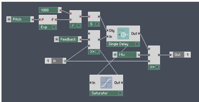
Fig. 12.2 The Structure of a comb filter.
