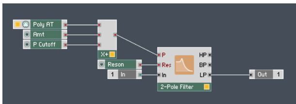
Fig. 2.46 The Structure for modulating a filter cutoff pitch with a Polyphonic MIDI Aftertouch signal.
