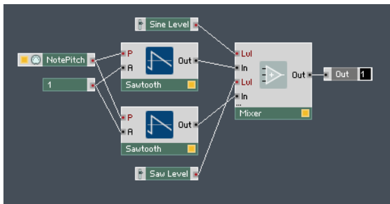
Fig. 5.23 For example, you can use the Mixer Module to mix two oscillator signals.
