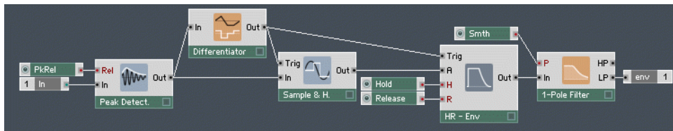
Fig. 10.2 The Structure for an envelope follower effect.
