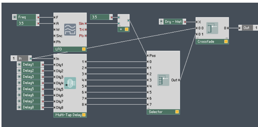
Fig. 11.6 The Structure for a scanning delay effect
