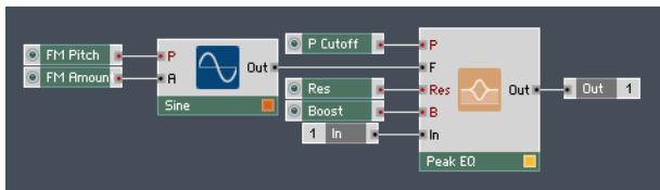
Fig. 10.29 A simple implementation of a peak equalizer.
