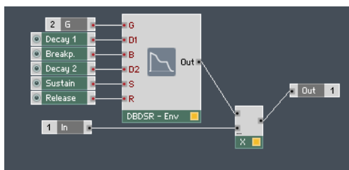
Fig. 9.26 A simple implementation of a decay-breakpoint-decay-sustain-release envelope.
