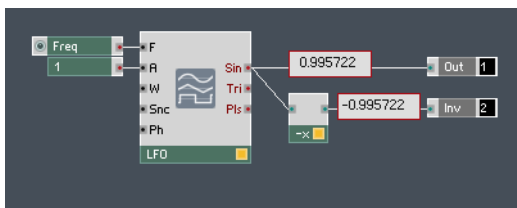
Fig. 4.9 The Invert Module changes the sign of the incoming signal.
