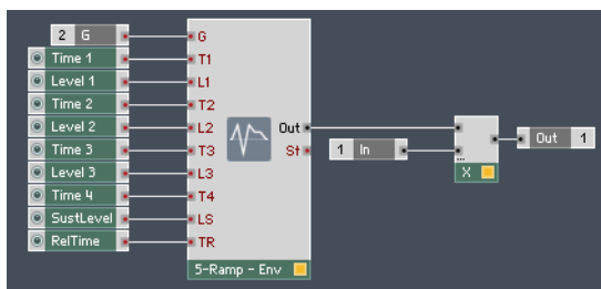
Fig. 9.56 A simple implementation of a 5-ramp envelope.
