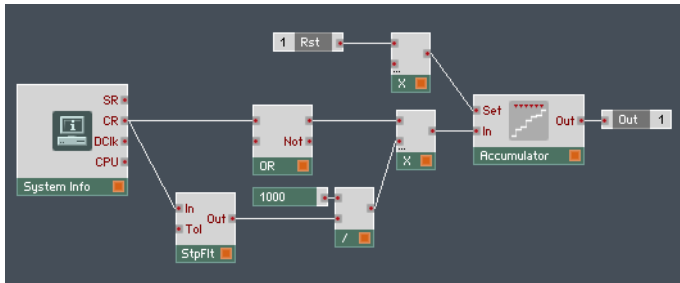
Fig. 13.42 The Structure for a simple Control Rate stopwatch.
