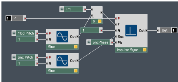
Fig. 6.81 A simple implementation of the Impulse Sync Module.
