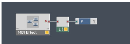
Fig. 14.13 The Event Voice Combiner All Module turns Polyphonic Event signals into Monophonic Event signals before outputting them from the Instrument.
