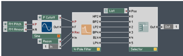
Fig. 10.15 A simple implementation of a 4-pole filter.
