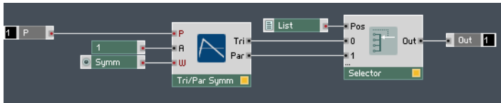
Fig. 6.26 A simple implementation of the Tri/Par Symm Module.
