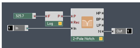
Fig. 4.40 Use the Log (F-to-P) Module to convert a precise cutoff frequency value to a logarithmic pitch value which is then fed to the "P" input port of a Filter Module.
