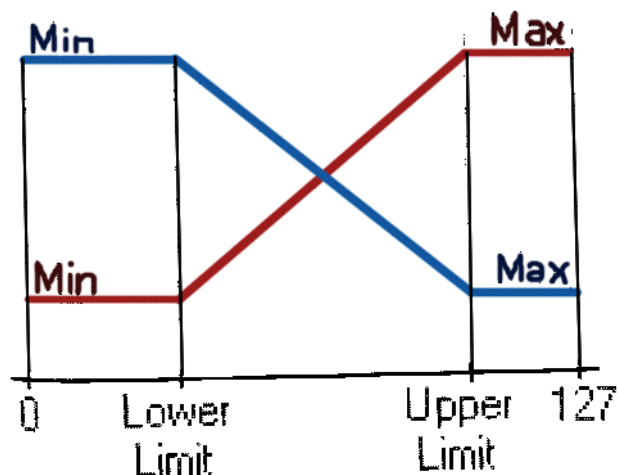
Fig. 2.11 The x-axis of the graph shows the incoming MIDI values whereas the y-axis shows the outgoing velocity values from the Gate Module. Setting opposite characteristics for two sources creates a crossfade effect between them, going from low to high MIDI velocity values.
