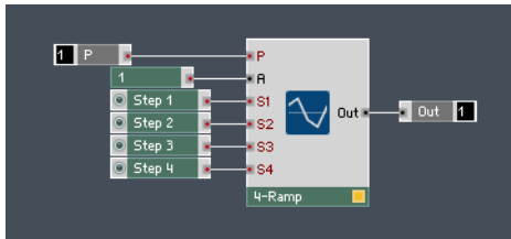
Fig. 6.96 A simple implementation of the 4-Ramp Module.
