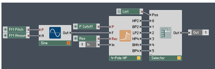
Fig. 10.18 A simple implementation of a 4-pole filter.
