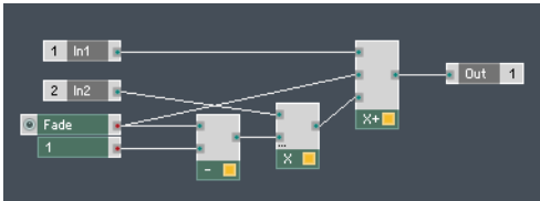
Fig. 4.16 The Structure for a simple crossfade effect.
