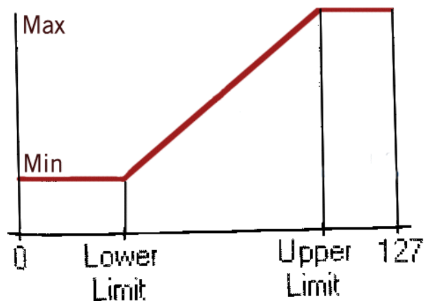
Fig. 2.25 The x-axis of the graph shows the incoming MIDI values whereas the y-axis shows the outgoing velocity values from the On Velocity Module. The values are interpolated linearly between “Min” and “Max”.
