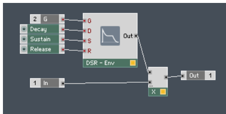
Fig. 9.20 A simple implementation of a decay-sustain-release envelope.
