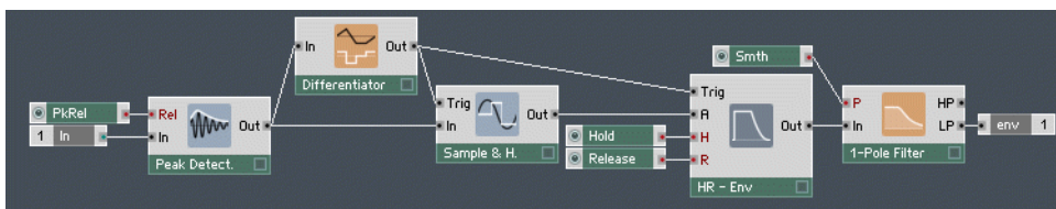
Fig. 12.36 The Structure for an envelope follower effect.
