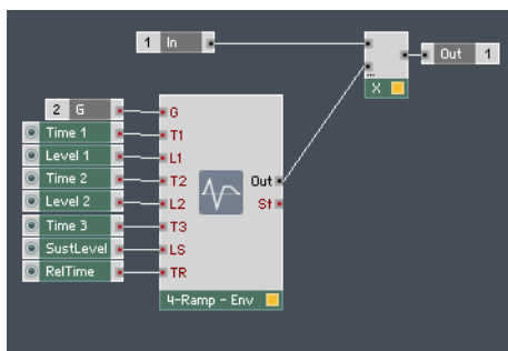
Fig. 9.53 A simple implementation of a 4-ramp envelope.
