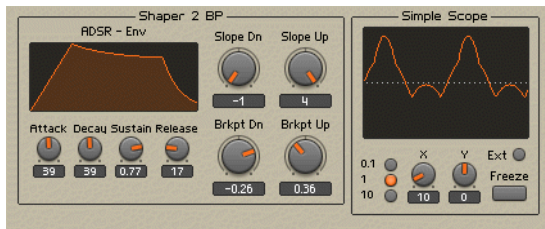
Fig. 12.23 The resulting waveform of a parabolic oscillator sent through a waveshaper with two breakpoints. Note the similarity to the Mirror 2 Module's effect on the same input signal. Here a positive slope value, "4", was used for the segment after the second breakpoint. That is why the upper part of the waveform is not mirrored.
