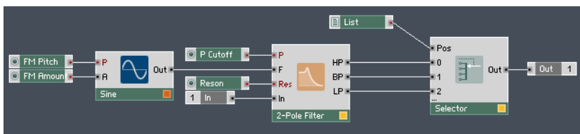
Fig. 10.9 A simple implementation of a 2-pole filter.
