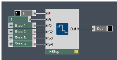
Fig. 6.84 A simple implementation of the 4-Step Module.
