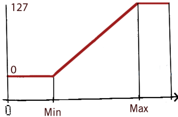
Fig. 3.2 The x-axis of the graph shows the values incoming at the "P" (pitch) input port whereas the y-axis shows the outgoing MIDI Note values. These values are interpolated linearly between over the interval [Min ... Max].
