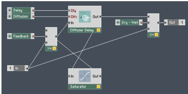
Fig. 11.9 The Structure of a simple diffuser delay effect.
