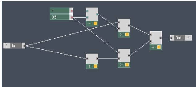
Fig. 11.17 The Structure of a very crude low-pass filter.
