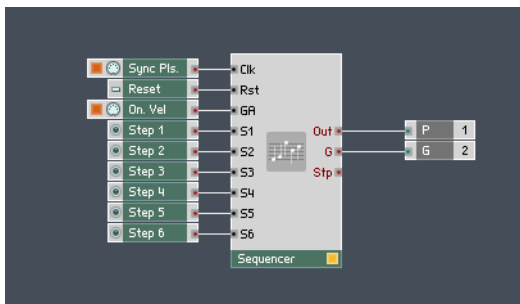
Fig. 2.64 The Structure for a 6-step pitch value sequencer.
