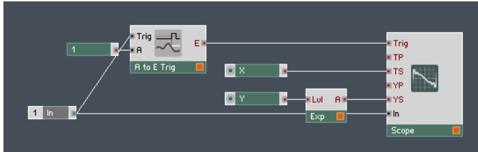
Fig. 1.54 The Structure for a simple scope that displays a Monophonic periodic Audio signal with regular zero crossings.
