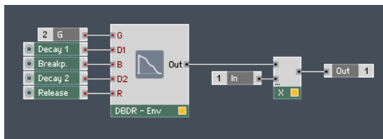
Fig. 9.23 A simple implementation of a decay-breakpoint-decay-release envelope.
