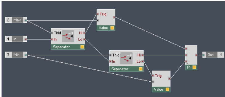
Fig. 13.36 The Structure for an Event clipper.
