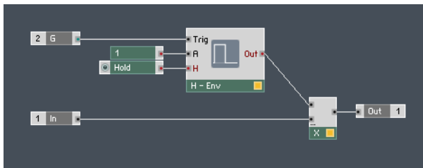
Fig. 9.7 A simple implementation of a hold envelope.
