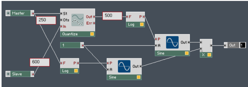
Fig. 4.31 You can use the Quantize Module to quantize the frequencies of a "slave" oscillator to a grid determined by the frequency of a "master" oscillator.
