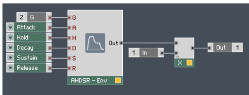
Fig. 9.47 A simple implementation of an attack-hold-decay-sustain-release envelope.
