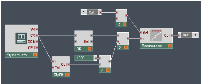
Fig. 13.2 The Structure for a simple Control Rate stopwatch.
