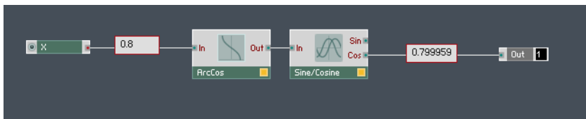
Fig. 4.55 ArcCos represents the inverse trigonometric function of the cosine function. When the two corresponding Modules are connected in series, they approximately cancel each other out.
