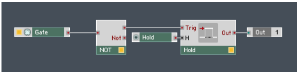
Fig. 13.53 Gate Off signals sent through the Logic NOT Module can be used to trigger Event processing, such as that of a Hold Module.
